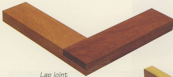
Lap joint
