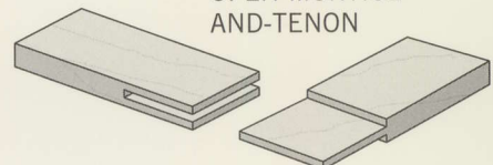
OPEN-MORTISE-AND-TENON
