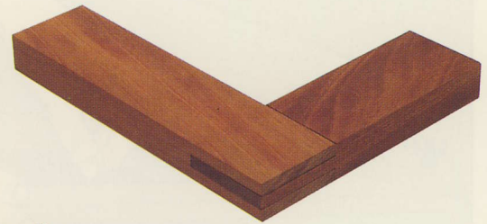
Open mortise-and-tenon joint
