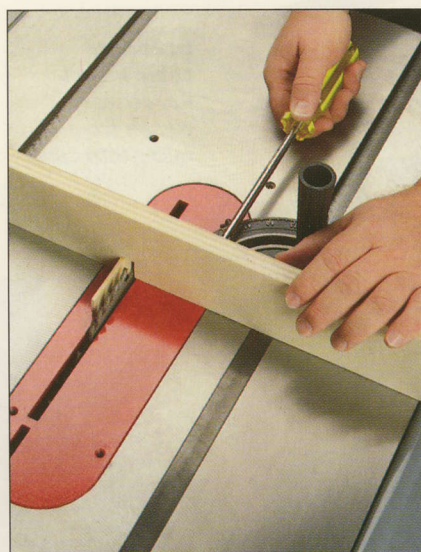
Screwed to the miter gauge, this wood extension facilitates the cutting of box joints for drawers and casework. Such shop-made jigs extend the versatility of the basic table saw.
