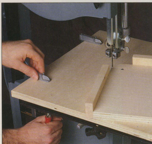
This quarter-circle-cutting jig is an ideal time-saver for rounding corners for tabletops. The jig pivots around a fixed point, taking the guesswork out of cutting perfect arcs.
