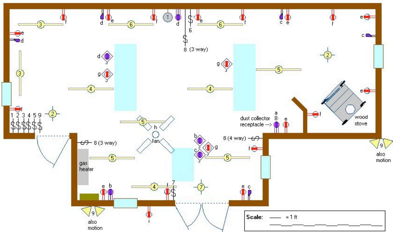
Electrical Layout for Frank Pellow's Workshop - Oct 7, 2004
