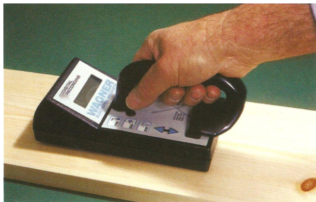
Figure 7.14* The electrode on the back of a dielectric meter generates a radio-frequency field as it is pressed against the face of a board. (Photo by Randy O'Rourke)
