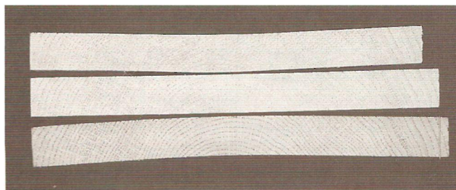
Figure 6.17 • Strips were cut in sequence from the end of an air-dry red oak board. As shown by the middle strip, it measured 91/2 in. wide at 14% MC. The top strip was then dried to below 4% MC—it both shrinks and cups. The bottom strip was allowed to readorb moisture to more than 20% MC. It expands and cups in the opposite direction. (Photo by Richard Starr)
