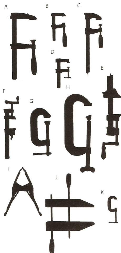
Figure 11.3 • Average clamping pressure of typical woodworking clamps. To find out just how much load each clamp could apply, Hoadley attached open steel frames to the crossheads of a universal timber-testing machine. With a clamp positioned to draw the frames together, the load applied was indicated on the machine. The clamps are described in the table, with the last column giving the average of three trials by an average-sized man. The quick-set clamp listed first in the table was used to calibrate the set-up: A secretary squeezed 330 lb., a hockey player squeezed 640 lb., and the author squeezed 550 lb. Repeated trials by each person yielded readings that agreed to within 10%. An asterisk indicates that the clamp began to bend, and the test was stopped at the value listed.
