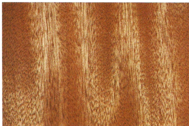
Figure 1.3 • The cells of mahogany are visible to the naked eye. In most species of wood, the cells are not as large and are visible only if magnified with a hand lens or microscope. (Photo by R. Bruce Hoadley)
