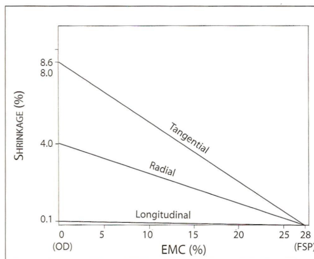
Figure 6.8 • Shrinkage vs. moisture content in northern red oak, a typical species.
