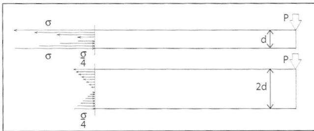
Figure 4.40 • In a cantilever beam, the maximum board stresses vary inversely with the square of the depth of the beam.
