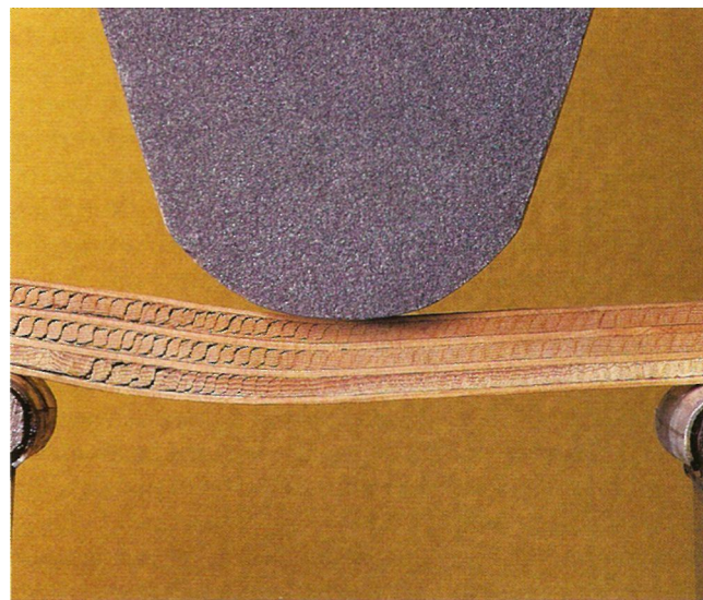
Figure 4.43 • Horizontal rolling shear, induced by lathe checks, develops when a 12-in. plywood beam is loaded in the center. This is analogous to putting weight on the edge of an overhanging plywood tabletop. (Photo by Randy O'Rourke)
