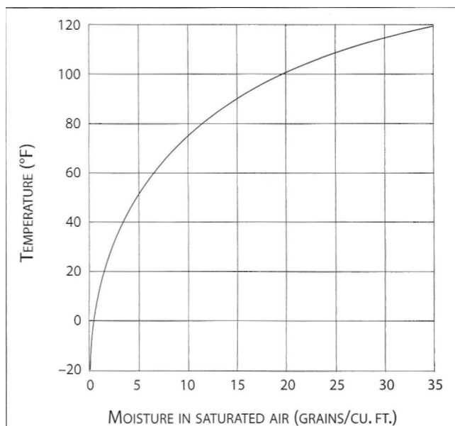
Figure 6.2 • The relationship between temperature and moisture content of saturated air. The maximum moisture that the air can hold depends on how warm it is; as the temperature rises, so does the saturation point.
