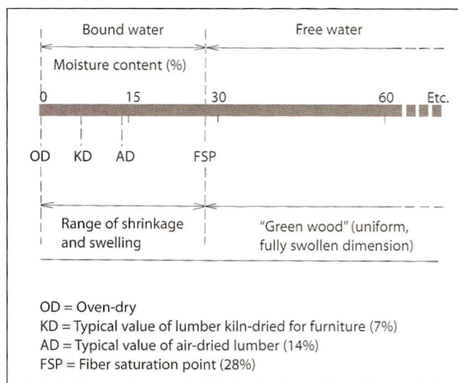
Figure 6.5 • Moisture-content values.
