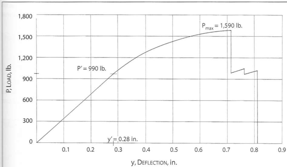
Figure 4.26 • A load/deflection graph for a white pine beam tested in static bending.
