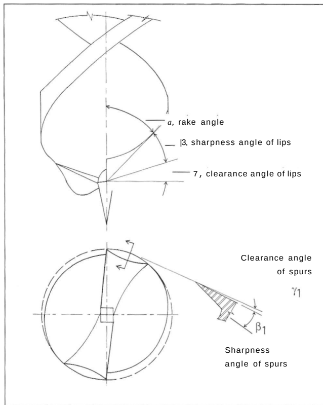
Figure 9.29 • The standard wood-boring bit has double spurs and double twist. The spurs, which have a fairly large rake angle and a slim sharpness angle, form the sides of the hole. The lips, with a rake angle of around 40^\circ and a clearance angle of 10^\circ to 15^\circ , follow behind the spurs to clear chips from the bottom of the hole.
