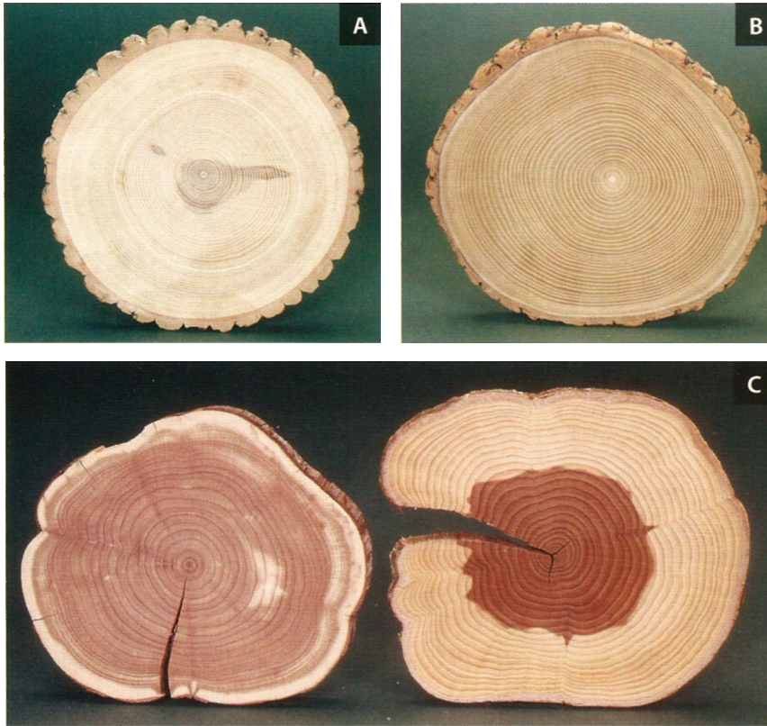
Figure 1.10 • The relative width of the sapwood varies according to species; heartwood (dark area) is small in white ash (A) and wide in catalpa (B). Heartwood/sapwood growth may also vary tremendously within a species, according to growing conditions. Both discs (C) were cut from eastern redcedar trees. The sample on the left was shaded by the larger trees around it reducing its crown. The one on the right grew normally in an open meadow with a full crown of foliage and greater need for sap conduction. (Photos by Randy O'Rourke)
