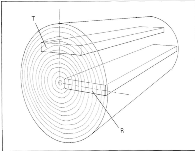
Figure 1.12 • In a flatsawn or flat-grained board (T), the growth rings are roughly tangent to the wide face of the board. In an edge-grained or quartersawn board (R), the rings are roughly perpendicular to the wide face.
