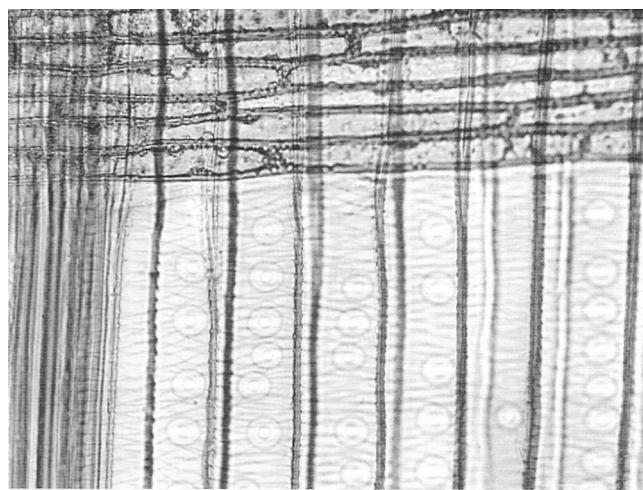
Figure 3.4 • Spiral thickenings on the inner walls of earlywood tracheids, the most definitive identification feature of Douglas-fir, appear under the microscope as fine coil springs. Even a tiny sliver can be positively identified by this constant feature. (Photo by R. Bruce Hoadley)
