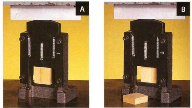
Figure 4.20 • The standard test for shear parallel to the grain is performed on a notched block (Figure 4.19) held in a special tool that keeps the sample from rotating while a blade (returned by springs) pushes straight down, shearing the block at the inside edge of the notch. (A) The sample is ready for testing. (B) The sample has failed in shear parallel to the grain. (Photos by Randy O'Rourke)
