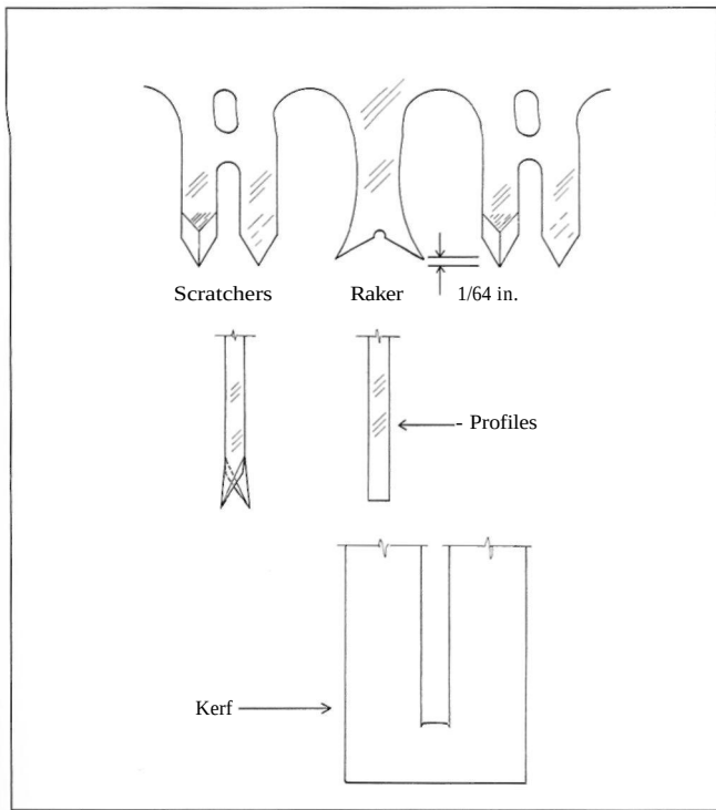
Figure 9.26 • The teeth on a classic two-man crosscut saw are ideally designed for their purpose. Spring-set scratchers filed to a spear point cut the fibers free at the edge of the kerf, then slightly shorter raker teeth come along to roll out the chips. Such a saw cuts when pulled in either direction.
