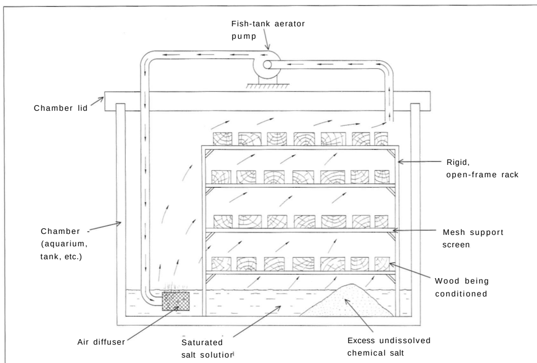
Figure 8.14 • An ordinary aquarium can be converted to a conditioning chamber for small wood samples. Passing air through a selected chemical salt controls relative humidity.
