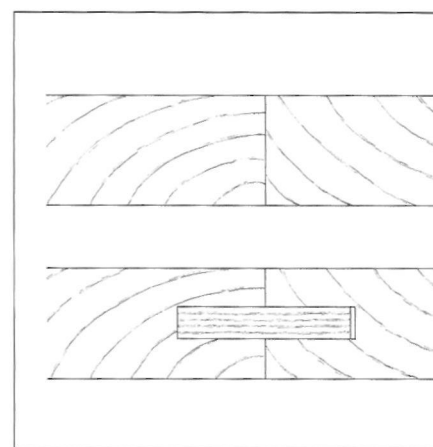
Figure 10.15 • Reinforcing an edge-glued joint with a cross-grain spline actually weakens the joint at the margins of the spline.
