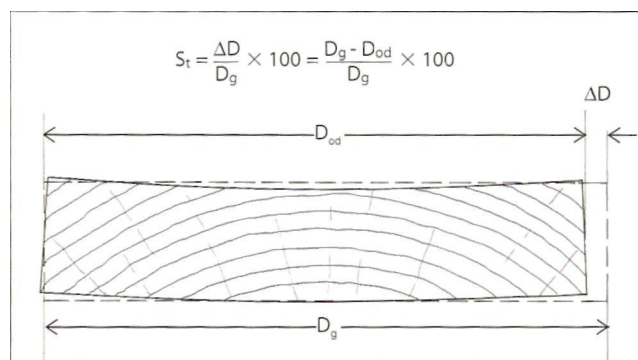
Figure 6.6 • The percent shrinkage (in this case tangential shrinkage, S_t ) is the change in dimension after oven-drying divided by the original dimension ( D_g ).
