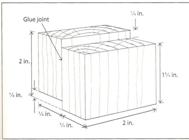
Figure 4.22 • The standard test specimen for measuring shear strength of a glue line is made of sugar maple. A special fixture holds the specimen in the testing machine in such a way as to direct the force along the plane of the glue line and prevent rotation of the block.
