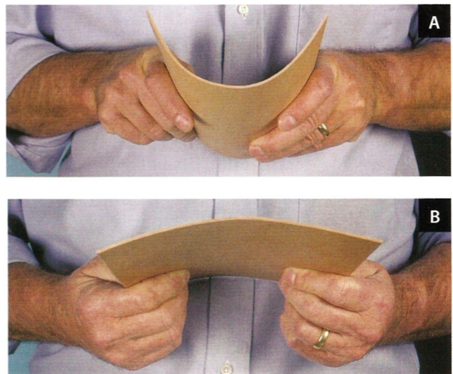
Figure 14.5 • Veneer flexes more easily when checks are opened (A) than when they are closed (B). This simple test distinguishes the tight and loose faces. (Photos by Randy O'Rourke)
