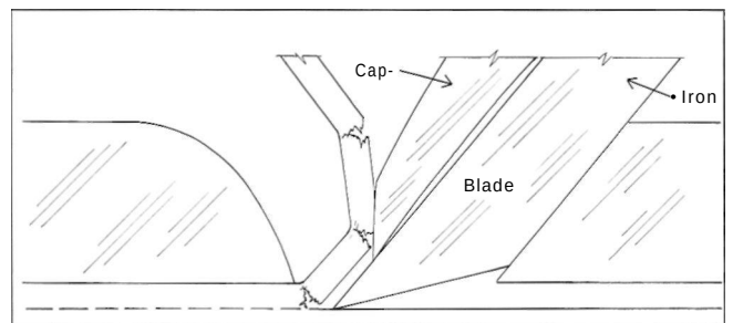
Figure 9.11 • In 90^\circ\text{-}0^\circ cutting with a handplane, the cap iron minimizes torn grain by breaking the chip near the cutting edge.
