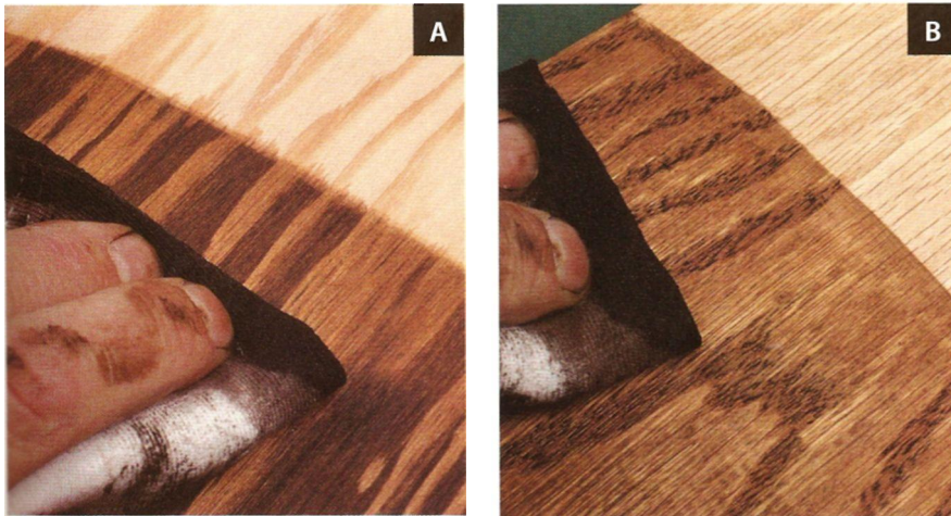
Figure 1.19 • Earlywood of Douglas-fir (A) is lighter in color than latewood but more porous. Thus it retains stain more readily and finishes darker in color. Large earlywood pores of red oak (B) already appear darker than those of latewood, and the effect is accentuated as the stain accumulates in them. (Photos by Randy O'Rourke)
