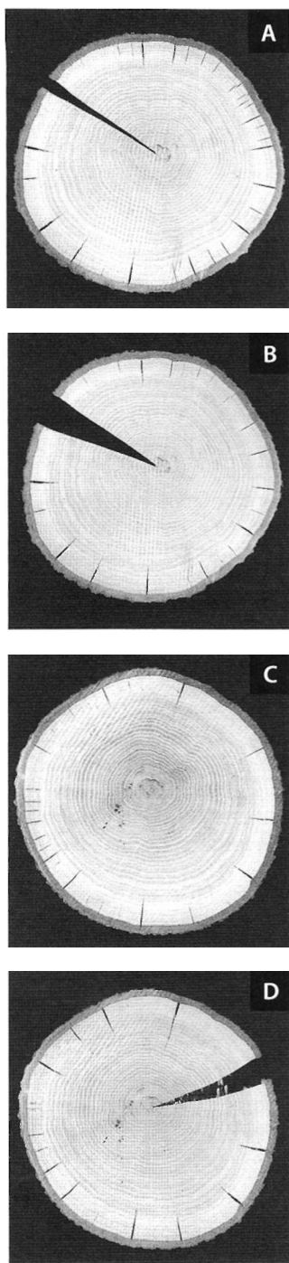
Figure 6.21 • Results of drying cross-sectional disks of northern red oak. This disk had a radial slot sawn in it (A). Because of heartwood extractives, the sapwood dries first and shrinks more, resulting in radial sapwood checks. When the heartwood dries, the slot opens wide (B). A disk without a slot (C) also forms sapwood cracks in early stages of drying. Eventual shrinkage stress opens a radial crack (D). (Photos by Richard Starr)
