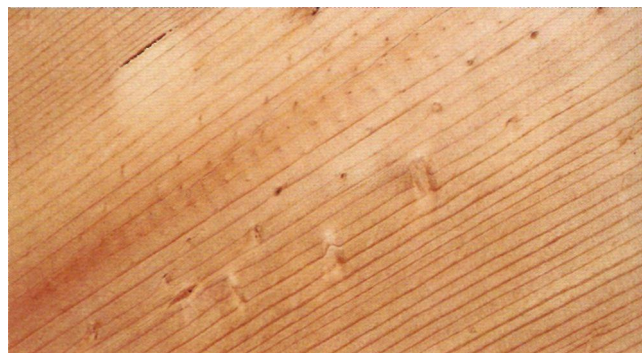
Figure 2.35 • Wide growth rings surrounding the pith (left) are juvenile wood, which is lighter and weaker than narrow-ringed mature wood. In the photo on the right, needle scars appearing as dots on the wood also indicate juvenile wood. (Photos by Randy O'Rourke)
