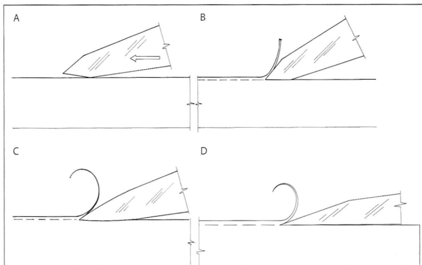
Figure 9.34 • The photo shows a new jackknife factory-ground to a large sharpness angle. It won't cut wood when held normally. The large sharpness angle results in a negative clearance angle (A). When rotated to eliminate the negative clearance angle (B), the cutting angle is so small that it's difficult to form a chip. Both faces of the blade must be lengthened to reduce the sharpness angle (C), or all the sharpening must be done on one face, keeping the other flat (D). (Photo by Randy O'Rourke)
