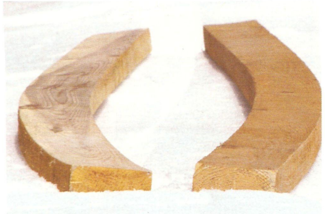
Figure 2.39 • Severe crook in roughsawn lumber caused by compression wood. (Photo by R. Bruce Hoadley)
