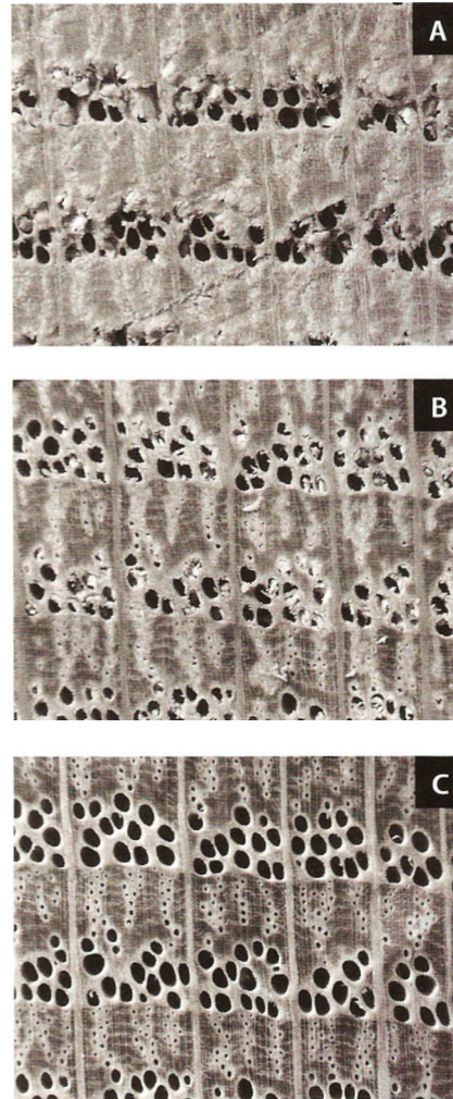
Figure 3.6 •The cleaner the cut, the more detail is revealed. Compare these cross sections of red oak that were cut with a saw (A), a dull razor knife (B), and a razor blade (C). (Photos by R. Bruce Hoadley)
