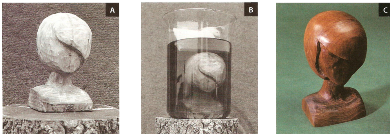
Figure 7.6 • This head (A) was rough-carved in a piece of cork tree ( Phellodendron sachalinensis ) and soaked for three weeks in a 40% solution of PEG-1000 (B). The treated piece was then dried in an oven at 212°F without checking and was finish-carved. The carving, 6 in. high (C), was finished with penetrating oil. (Photos A and B by Richard Starr; photo C by Randy O'Rourke)
