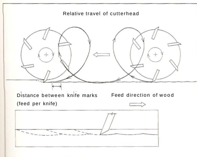
Figure 9.12 • In peripheral milling, each cutter follows a trochoidal path relative to the workpiece, the result of cutterhead rotation plus feed. Each cutter takes a curved chip from the workpiece, usually by up-milling (inset).
