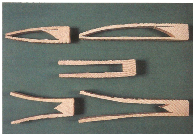
Figure 8.7 • Stress sections evaluate stress distribution in lumber. In the center piece, parallel prongs indicate a stress-free board. On the top, prongs curve inward, indicating case-hardening. On the bottom, prongs spread outward as the result of reverse case-hardening. (Photo by Randy O'Rourke)
